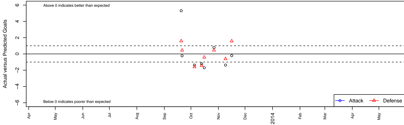
SRU Celtic B02 Dots are actual minus expected GF (blue circles) and GA (red triangles). Blue line is smoothed change in attack strength. Red is smoothed change in defense strength.
